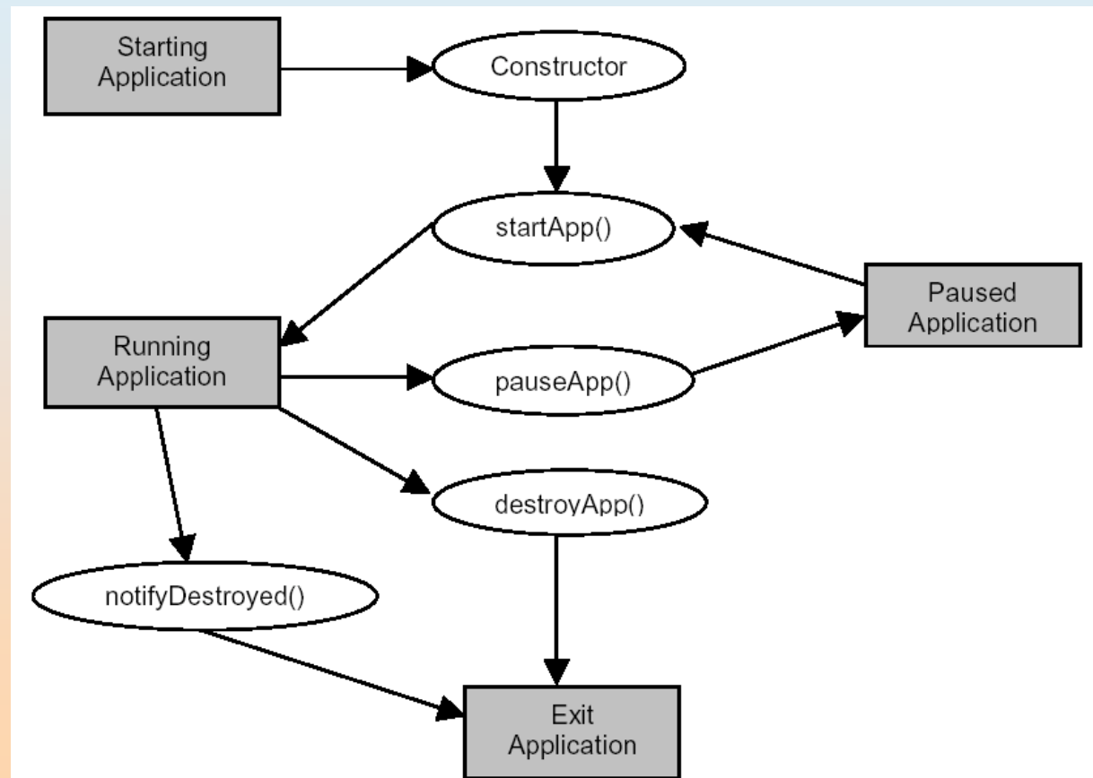
Midlet life cycle
